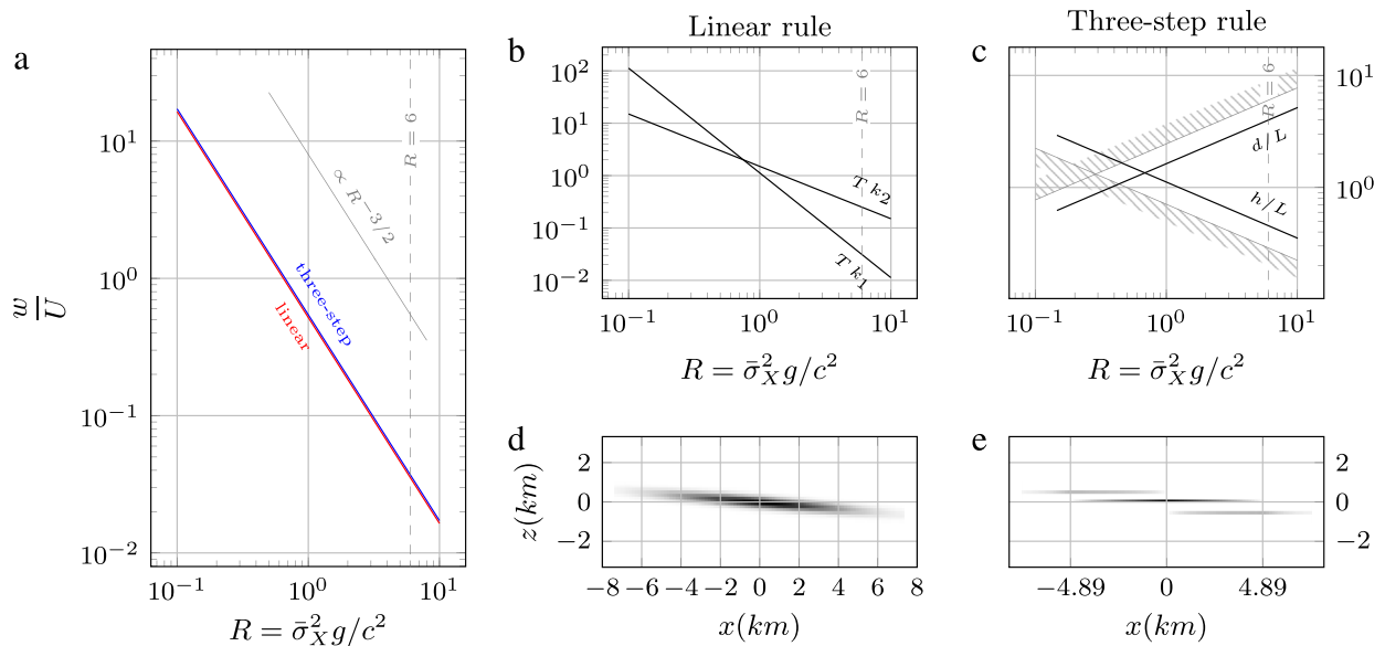
Fig. 4. Comparison of control rules: (a) control cost w = \mathbb{E}[|u|_1] as a function of the dimensionless parameter R for the two different control rules; the two control costs are almost indistinguishable, differing by less than 5%. (b,c) Control parameters and (d,e) corresponding probability density for the hurricane case ( R = 6 ) for the linear and TLC control rules. Gray patterns in (c) define the limit of each curve for which a given value of R is attainable, given by (14).
