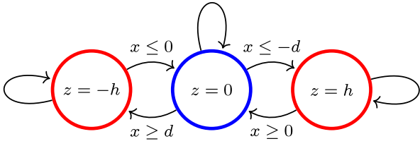
Fig. 2. Implementation of the three-level control rule.
