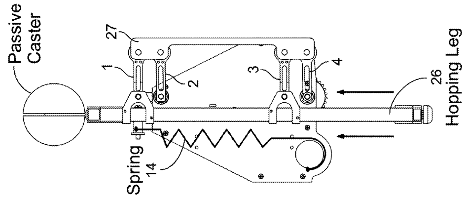
Upright State FIG. 6C
