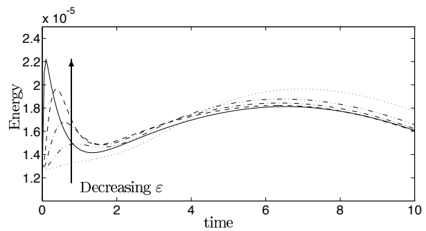
Figure 2: Energy evolution of controlled cases with linear control for different values of the penalty parameter \varepsilon = 0.01, 0.05, 0.1, 0.2, 0.5 as solid, dash, dash-dot, dash-dot-dot, dot respectively.
