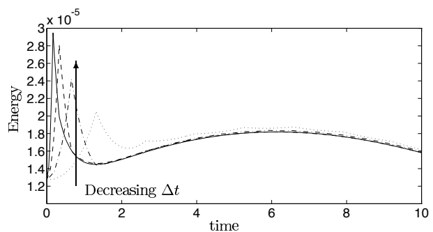
Figure 3: Energy evolution of optimally controlled cases with non-linear control for different time resolution of the control. Using 300,150,75,37 degrees of freedom in time as solid, dash, dash-dot, dot respectively.
