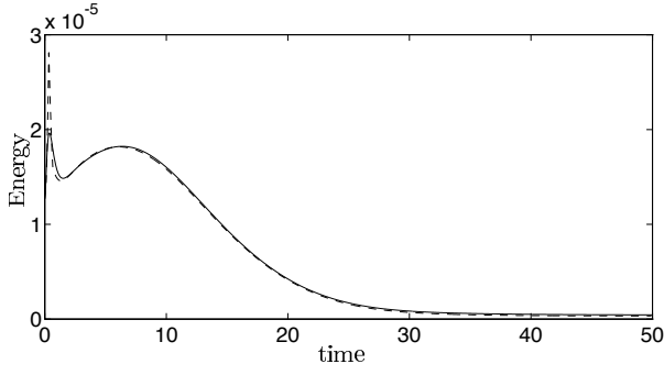
Figure 4: Energy evolution of optimal linear control case with \varepsilon = 0.05 (solid) and optimal non-linear control with 150 degrees of freedom in time (dash).
