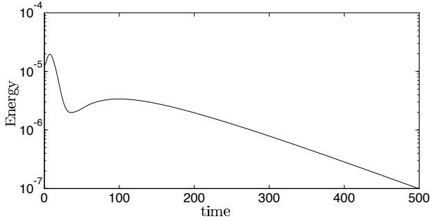
Figure 5: Energy of state error in estimation for \alpha = 0.01 .
