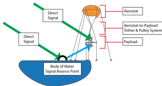
Figure 4. Tethering configuration overview.
