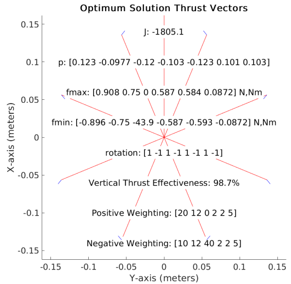
Figure 6. An excursion to utilize the optimizer for X8 octorotor design
